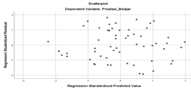
Gambar 1. Scatterplot
