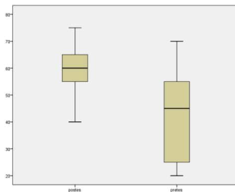
Gambar 2. Box-plot
