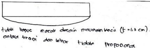
Figure 6 AL Written Results when Explaining ideas
